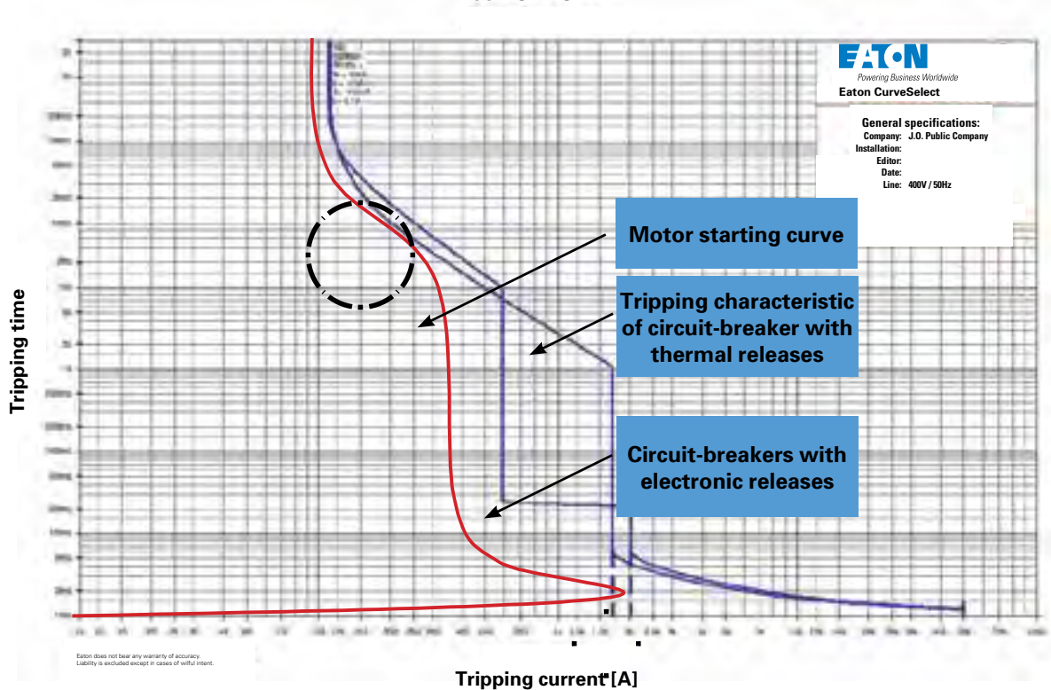
Figure 3: Circuit-breakers with electronic releases enable – by flexible setting features – a more exact matching to the typical current consumption curve of a starting three-phase motor than is possible with the switch on thermal overload releases.
