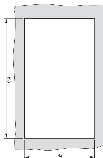
Mounting dimensions
