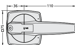
Type K2D & K2SD - versions available for both 6mm + 8mm square shafts
