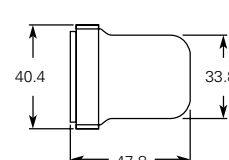
Transparent flexible boot for illuminated pushbutton Catalogue no. 10250TA25
